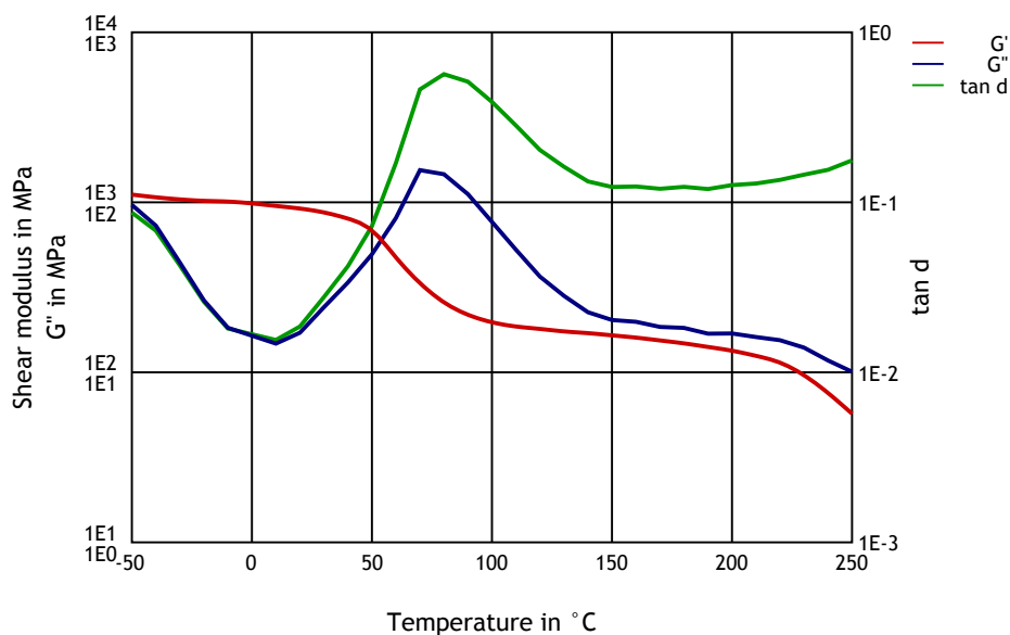
Dynamic Shear modulus-temperature (dry)
