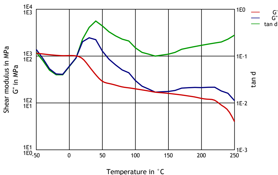
Dynamic Shear modulus-temperature (cond.)
